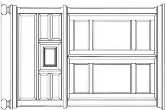
-045 Armoire Deck W44" x D22" x H72" I.D. W39 1/2" x D19-1/4" x H33"
