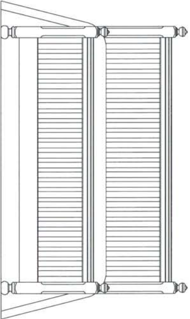
King or Queen Size -250 5/0 Hd/Bd — W66" x D4" x H60" -251 5/0 Ft/Bd — W66" x D4" x H35" -270 6/0, 6/6 Hd/Bd — W82" x D4" x H60" -271 6/0, 6/6 Ft/Bd — W82" x D4" x H35"
