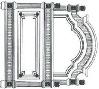
-530 3/3 Panel Bed Hd/Bd — W42" x D4" x H54" -531 3/3 Panel Bed Fv/Bd — W42" x D4" x H33" -401 3/3 Bed Rails w/ support system -532 4/6 Panel Bed Hd/Bd — W58" x D4" x H56" -533 4/6 Panel Bed Fv/Bd — W58" x D4" x H33" -402 4/6 Bed Rails w/ support system
