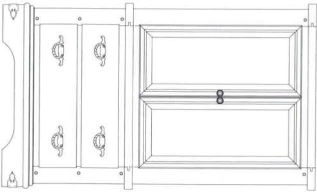
-045 Armoire W41" x D22" x H69" 2-Adjustable Shelves Inside Dimensions: W37 1/4" x D18 3/4" x H36 3/4"
