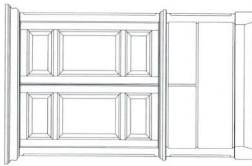
-045A Armoire Deck W42" x D22" x H45" -045B Armoire Base W40" x D21" x H26"
